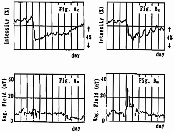
Examples of Forbush Decreases (Deep River)
