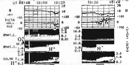
Figure 1 Two examples of different solar wind injections in the distant magnetopause between the magnetosheath and lobe. Each subset with multi-panels shows magnitude and directions ( \theta and \phi ) of the magnetic field, and omni-directional energy-time diagrams of electrons and ions detected by the LEP-EA-ele, EA-ion, and SW sensors from the top, respectively. GEOTAIL moves from the northern lobe into the magnetosheath in both of the examples. (a) O^+ can be found together with the CDIF in the lobe, as indicated by an arrow at a left-hand ordinate of the EA-ion panel. The lowest diagram shows that two-branch H^+ streams exist in the boundary (thick underline). (b) The CDIF is coupled with the solar wind, while there are no two-branch proton streams.
