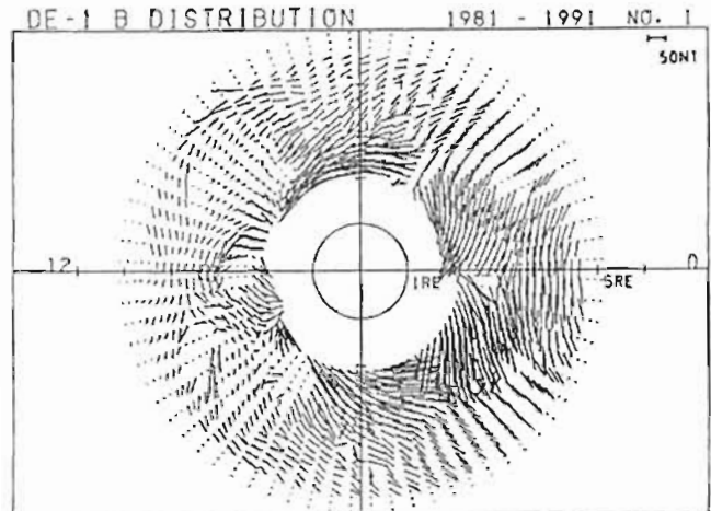
Fig.1 ΔB vectors at the centers of volume elements in the noon-midnight meridian plane. The z-axis is along the earth's magnetic dipole axis.
