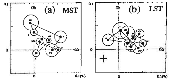
Figure 1. Harmonic diags of the sidereal diurnal variations observed by 9 component telescopes in each of Matsushiro(a) and Liapootah(b) in three years from January 1992 to December 1994. Error circles are deduced from the dispersion of three yearly-mean vectors.
