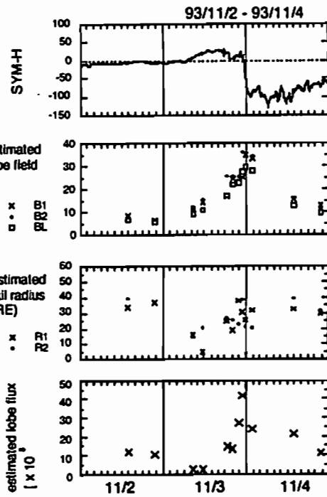
Figure 1. Changes in tail during November 3-4, 1993 storm. The four panels show SYMH (1min Dst), estimated (B1, B2) and measured (B1) lobe field strength, estimated tail radius of the tail and estimate lobe flux for November 2-4, 1993. The numbers 1 and 2 correspond to intervals just before and after the lobe entry.
