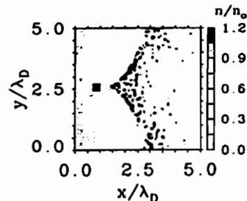
図2: Simulation results of the spacecraft-plasma interaction. (from Okada, et al., 1993, in print)
