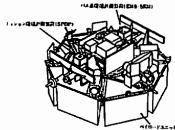
図1: Configuration of SFU Experiment. (from Sasaki, S. et al., 1993)
