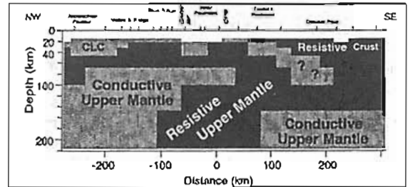
Fig. 2 Simplified resistivity model for the line 300.
