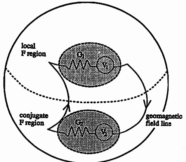
Figure 1. Electric circuit model of conjugate F regions.
