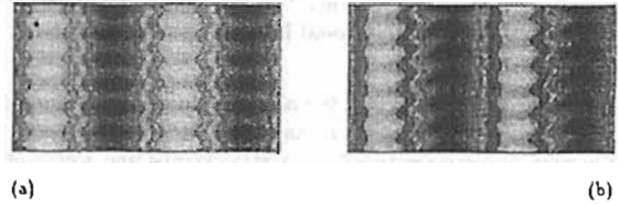
Figure 1. Contour map of the field line integrated Pedersen conductivity in the plane perpendicular to the geomagnetic field. The size of the calculation is 125x125 km. The horizontal and vertical lines are east-west and north-south direction, respectively. The initial condition is shown in (a) (b) is 10 min. after the start.
