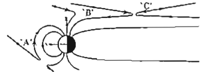
Figure 2 Solar wind injections in the dayside ('A'), the mantle ('B'), and distant tail lobe ('C')
