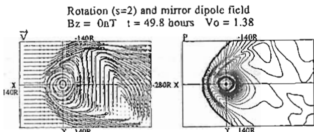
Fig.2. Velocity and plasma pressure distribution on the
