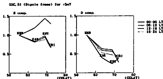
Fig. 1 Latitudinal profile of the amplitude of SSC and SI (normalized to the MIB amplitude)
