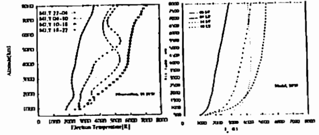
Fig. 1. Observed and modelled T_e profiles.
