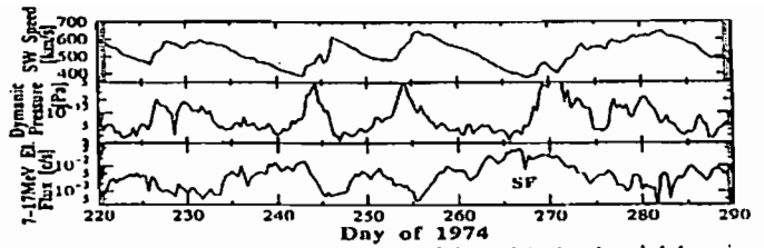
Fig.1 Comparison of 8-hour averaged solar wind speed (top), solar wind dynamic pressure (middle), and 7-17MeV electron flux (bottom) measured by Pioneer11. "SF" indicates solar flare particle event.
