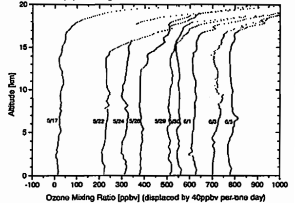
Figure 2. Tropospheric Ozone Profiles in May and June 1995 The tropopause height was about 17km.
