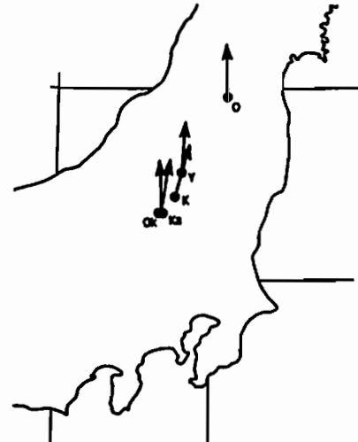
Fig. 1. The mean paleomagnetic directions for Miocene (15Ma-6Ma) welded tuff formations. Arrows indicate the declination for the Ohsawa (O), Yatakezawa (Y), Kinugawa (K), Katashinagawa (Ka) and Okkai (Ok) formations.
