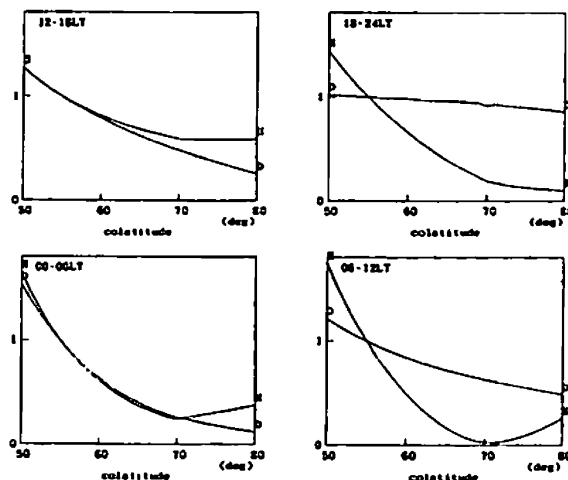
Fig. 2 Latitudinal variation of magnetic field obtained from model calculation of ionospheric current system (normalized to the amplitude at 55° colatitude)
