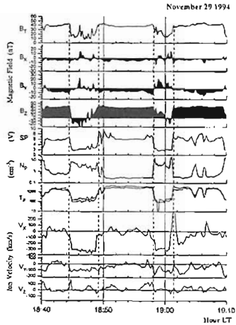
Figure 1. Transient events observed on November 29, 1994. SP, Np, and Tp denote the satellite potential (volt), ion density (/cm 3 ), and ion temperature (eV), respectively. The time resolution of the data is 12 seconds.
