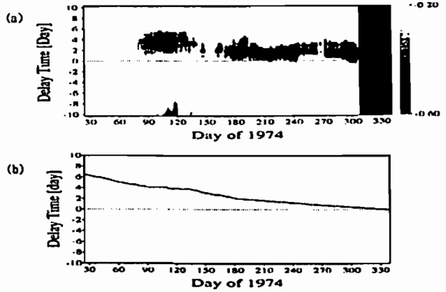
Fig.2 (a): A dynamic cross-correlation between electron flux and solar wind dynamic pressure. The analysed data set is name as Fig.1. Data points are selected by criterion that coefficient is less than -0.4. The blank portion indicates the period when Pioneer11 is in Jovian magnetosphere, and irregularity around day270 is caused by solar flare effect. (b): The solar wind propagation time from Pioneer11 to Jupiter estimated by the in-situ solar wind speed and position of Pioneer11 and Jupiter.
