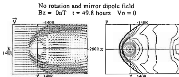
Fig.1. Velocity and plasma pressure distribution on the equator for no rotation and mirror dipole field.
