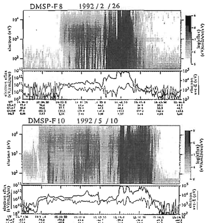
Figure 1. Energy-time spectra of precipitating electrons observed by the DMSP satellites on (top) February 26 and (bottom) May 10, 1992. Both intervals are after substorm onsets at the main phase of magnetic storms. Subauroral intense electron precipitations are observed at the low-latitude part of the precipitation regions.
