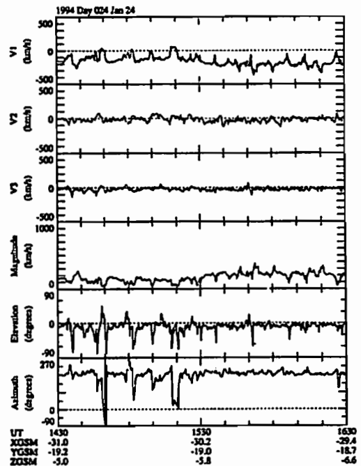
Figure. Ion bulk velocity oscillations in the boundary layer.
