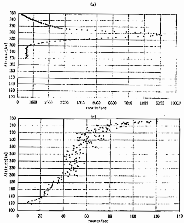
Fig.1 Counting rates versus scanning altitude (a) on upleg. (b) on downleg. Below 220km, scanning operation was carried out.
