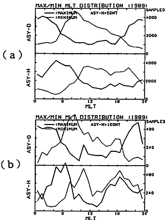
Fig. 1 Local-time distribution of the stations which give the maximum or the minimum value of the disturbance fields. (a) and (b) correspond to the moderate and large disturbances measured by the ASY-H index, respectively.
