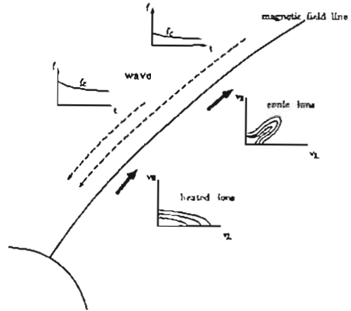
Fig.1: Waves - ion conics interaction model
