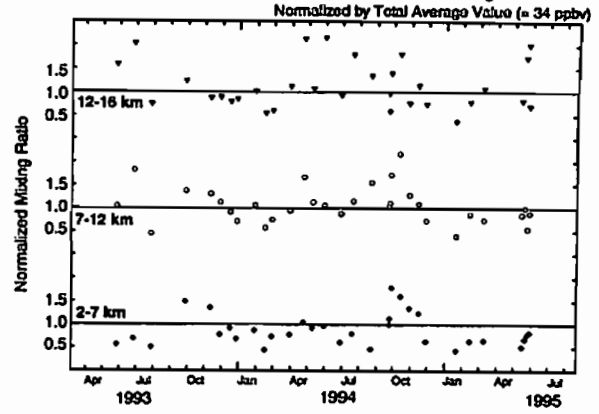
Figure 1. Seasonal Variation of Tropospheric Ozone Mixing Ratio
