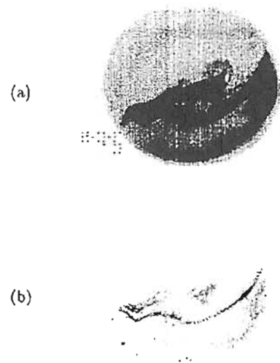
Figure 1. An example of images of all-sky camera on 11:17 03, Feb 28, 1995. (a) is an image of total lights and (b) is that of 670.5nm. Active aurora arcs are seen near the zenith of the sight both in (a) and (b). Slight enhancement of aurora is seen near the bottom side.
