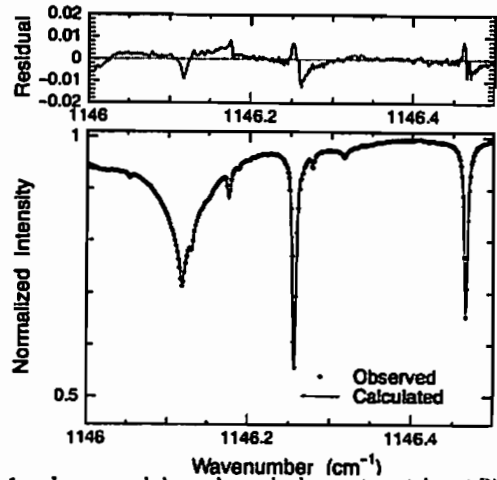
Figure 1. Lower panel shows observed solar spectrum taken at Rikubetu at 16:00-16:05 JST on July 19, 1995, at spectral region of 1146.0-1146.5 cm -1 (black dots) with resolution of 0.0035 cm -1 , while the calculated spectrum (solid line) by SFIT program is overlaid. Upper panel shows the residual of the calculation compared with the observation.
