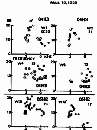
Fig. 3 Temporal variation of polarizations.
