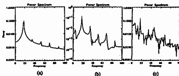
Figure 3: Frequency power spectra of enstrophy for different dissipative coefficients. Cases (a), (b) and (c) correspond to Simply Periodic, Doubly Periodic and Chaotic regimes, respectively.
