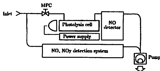
Fig. 1 Schematic diagram of the NO 2 photolysis system using metal halide lamp.
