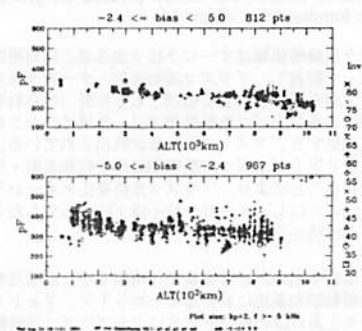
Figure 1: Bias voltage dependence of antenna capacitance
