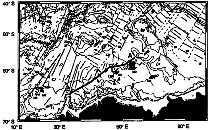
Fig. 1 Fracture zones and magnetic anomaly lineations in the Southern Indian Ocean. Dashed and solid lines show previously identified fracture zones and magnetic anomaly lineations (Cande et al., 1989). Stippled and thick solid lines indicate fracture zones and magnetic anomaly lineations determined from vector geomagnetic anomaly field data as well as sea surface and satellite gravity anomalies. Bathymetry contour is based on ETOPOS.
