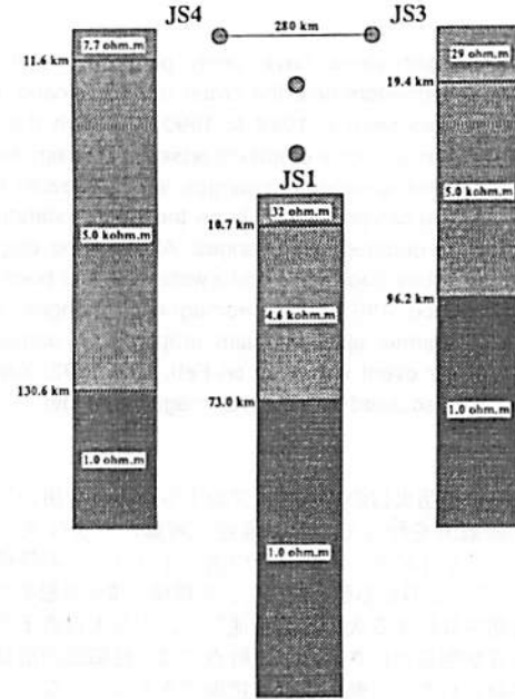
Fig. 1 1D conductivity structures of the Pacific plate at sites JS1, JS3 and JS4 derived by the observed VGS estimates.
