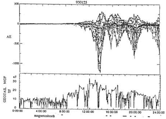
Figure 1 Horizontal component of the high-latitude magnetograms, GEOTAIL magnetic field data of January 25 1993
