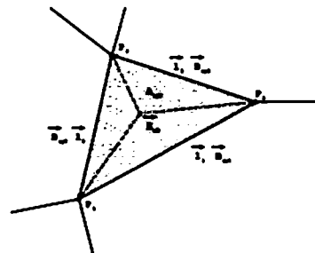
図1: Discretization of the \nabla \times \vec{B}_n component.
