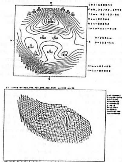
Fig. [O1]630.0nm intensity contour-map in 02:23:06 LT, February 21. Assuming the emission layer-height 250km, the radius is 767km.
