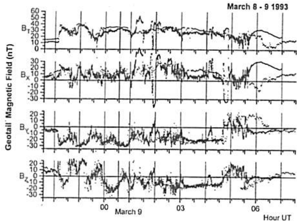
Figure 1. Time for GEOTAIL data is shifted by 34 min taking into account an approximate propagation time of IMF effect to the distant tail.
