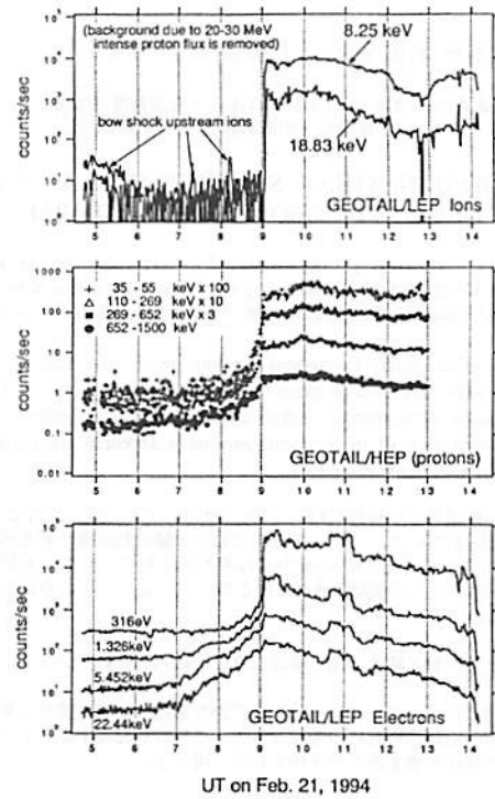
Fig. 1a (top): Counting rates of the suprathermal ions (LEP/EAI). Before 0903 UT, no interplanetary-shock related ions were observed in the energy range below \sim 30 keV/q. Ions observed before 0540 UT, around 0720 UT, and 0815 UT were those typically found in the bow shock upstream region.
