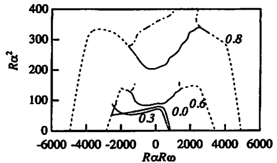
Figure 1: Marginal stability curves for model M2 for dipole family. The numbers 0.0 to 0.8 at the curves denote the ratio of inner radii. Solid line, dotted line, and dash-dotted line represent primary stationary mode, primary oscillatory mode, and secondary stationary mode, respectively.
