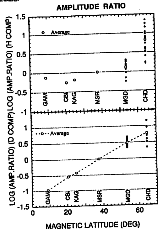
Fig.1. Pi 2's ratio of amplitudes with respect to Moshiri observed at northern stations (Guam, Chichijima, Kagoshima, Moshiri, Magadan, and Chokurdakh) of the 210° MM chain.
