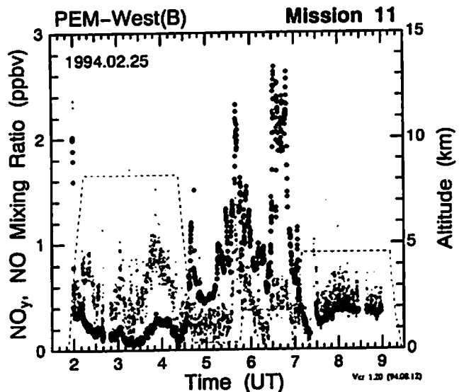
Figure 1. Measured mixing ratios of \text{NO}_y (•) and \text{NO} (x) in addition to flight altitudes (broken line). Scale of NO should be divided by 20.
