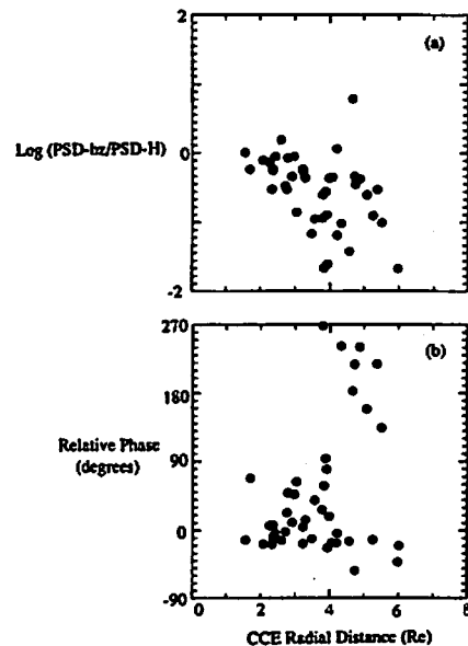
(a): The spectral density of magnetic field magnitude at CCE normalized to that of the Kakioka H component at the frequency of a Pi 2 pulsation seen at Kakioka, as a function of radial distance of CCE. (b): Same as (a) except that the relative phase is taken as the variable.
