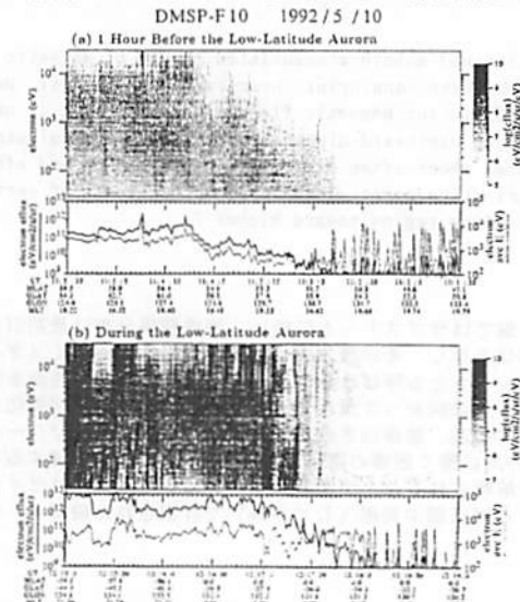
Figure 1. Energy-time spectra of precipitating electrons observed by the DMSP-F10 satellite (a) at 1 hour before the appearance of the aurora and (b) during the appearance of aurora, on May 10, 1992.
