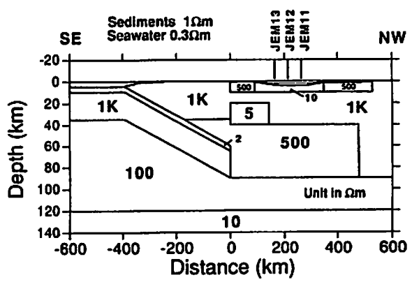
Optimum 2-D Model beneath the Tsushima Basin
