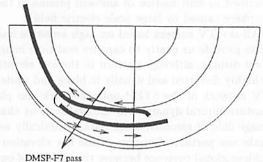
Figure 1. Schematic view of the two arc formation event.
