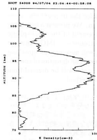
Fig.1 The mesospheric potassium profile measured by the Ti:sapphire laser.
