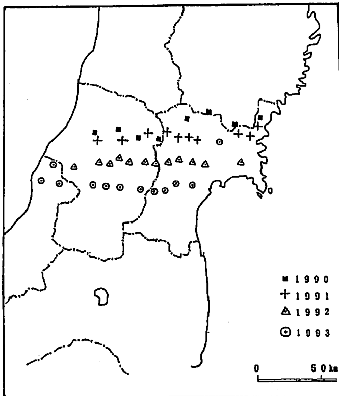
Broad-band magnetotelluric sounding along the three transects.
