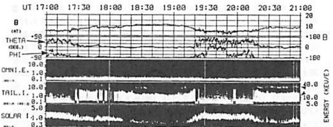
Figure 1 Magnitude and directions of the magnetic field and Energy-time diagrams of electrons and ions. Ion spectra are measured simultaneously by two sensors of different energy ranges and acceptance angles; LEP-EAi and LEP-SW. In the magnetosheath, since energy mode of EA is changed from wide-energy range (32eV/q-40keV/q) to high-energy range (5-43keV/q), the data obtained by the SW sensor should be referred.
