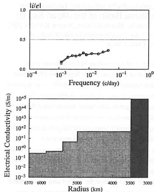
Fig. 1. Response function and a determined electrical conductivity profile in the mantle.
