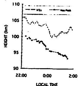
Fig.3 Temporal variation of the height of Nas layers and the height of Es layers.
