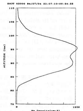
Fig.2 The mesospheric sodium profile measured by the dye laser simultaneously.
