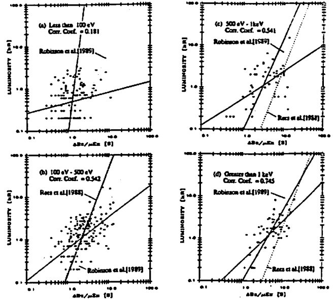
Relationship between auroral luminosity and \Delta Bz/\mu E_z for the characteristic energies: (a) less than 100 eV, (b) 100 - 500 eV, (c) 500 - 1 keV, and (d) greater than 1 keV.
