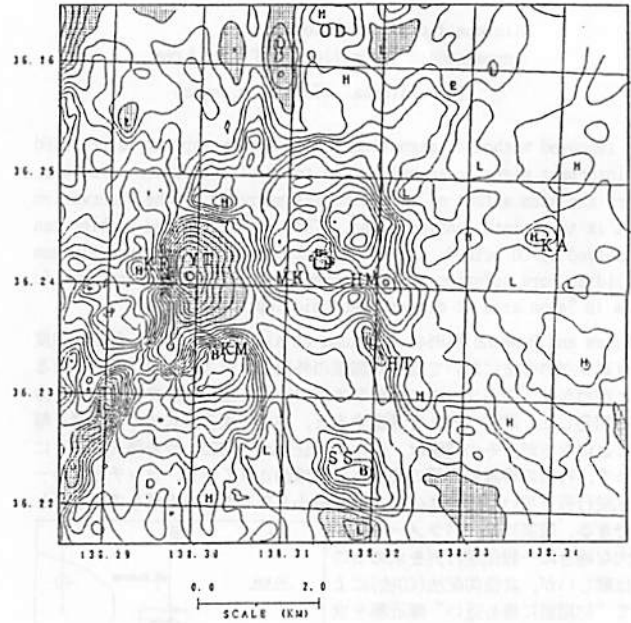
ASAMA MAGNETIZATION INTENSITY
