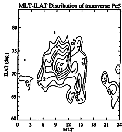
Figure 1. MLT-ILAT distribution of occurrence probability. The probability is given by the occurrence number of transverse Pc5 divided by the number of orbits in each mesh of one hour of MLT by 2 degrees of ILAT. The numerals indicated on contour lines represent roughly one half of the probability in percentage. The actual probability is at least double the indicated number because the average duty cycle of the DE-1 magnetometer is less than 50 %. We can see a strong dawn/dusk asymmetry in the distribution.
