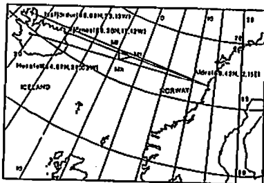
Fig.1 Propagation path of VLF signals: Omega Aldra-Tjörnes, Isafjörður and Husafell, Iceland. Mt, Mi and Mh are the middle points of Tjörnes to Aldra.
