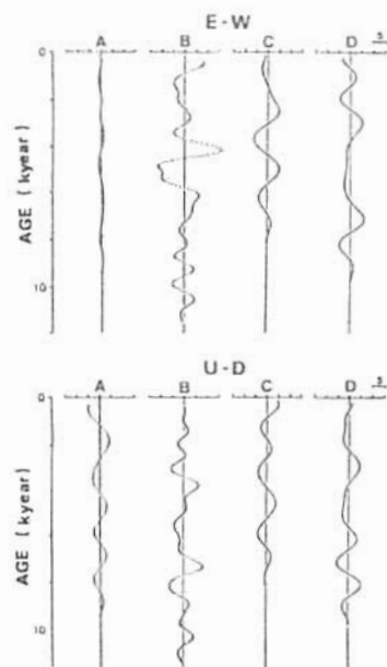
Fig.1 The secular variation components of band periods ca.3000 yrs for the records from Australia(A), Japan(B), N. America(C), and Great Britain(D). Variations are defined by the angles from the axial dipole field directions of each site.
