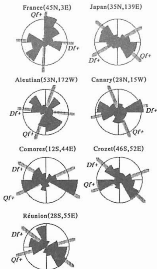
Fig.2 Rose diagram of relative azimuth of Brunhes VGPs.
