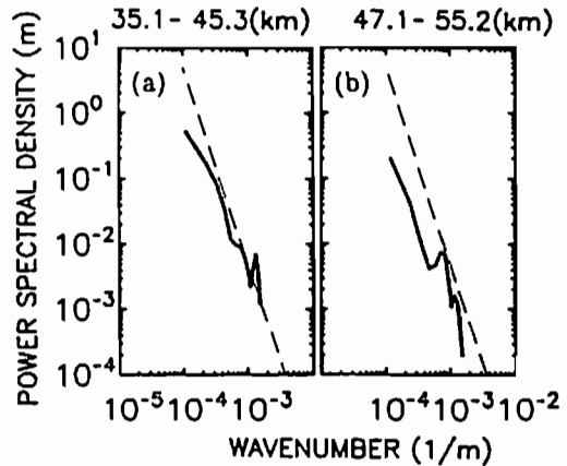
Figure: Vertical wavenumber spectra of normalized temperature fluctuations observed by a rocketsonde on 17 January 1990. Solid lines indicate observed spectra in (a) the upper stratosphere and (b) lower mesosphere, while dashed lines show the model spectrum.
