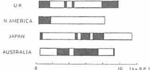
Fig.1 The secular variation components of band periods ca.3000 yrs for the records from Australia(A), Japan(B), N. America(C), and Great Britain(D). Variations are defined by the angles from the axial dipole field directions of each site.
