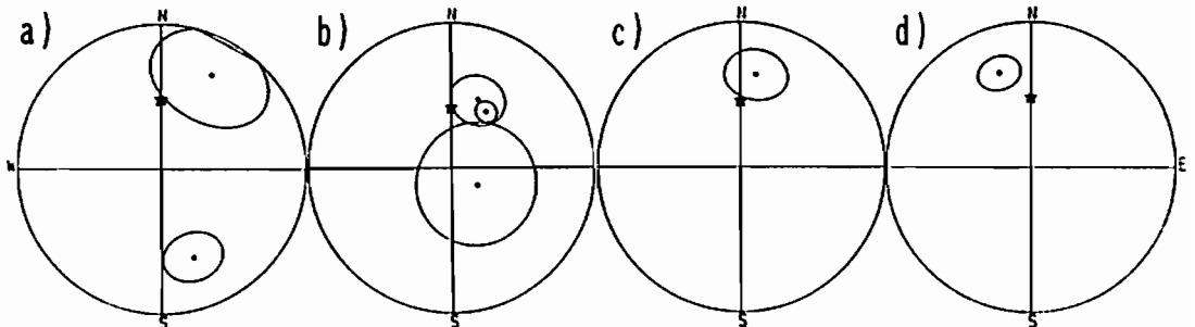
Fig. 8. Site-mean characteristic directions before tilt corrections. Ellipses are 95% confidence circles of equal-area projections. Star symbol is the direction of the geocentric dipole field (GDF) for the sampling locality. a) Cambrian; b) Devonian; c) Permian; d) Triassic.
