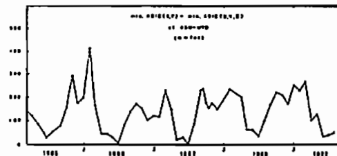
Fig.3 Monthly variation of the difference in ABIC values between the above two cases.
