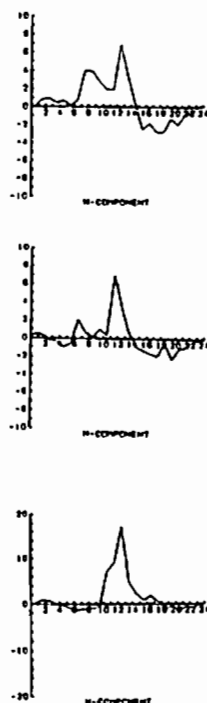
Fig. 2. Difference of the geomagnetic H component, when IMF-By > 0 and < 0 at Sabhawara (geomagnetic lat. 21^{\circ} N, top), Aibag ( 10^{\circ} N, middle) and Trivandrum ( 1^{\circ} S, bottom) in 1980.
