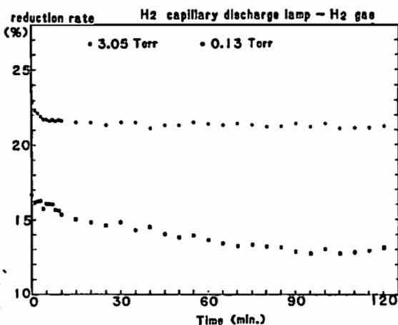
Figure 1 Temporal change of absorption with keeping a filament temperature at 1100°C. The data in the figure were obtained by using a H 2 capillary discharge lamp as a source and H 2 gas in a cell.
