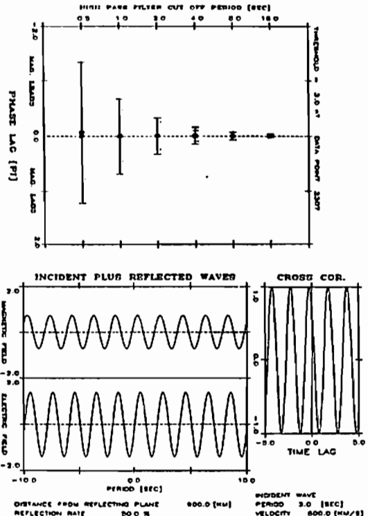
Upper panel : Standard deviation of peak distribution of cross-correlation using some high-pass filters Lower panel : Model calculation of Alfvén wave reflection
