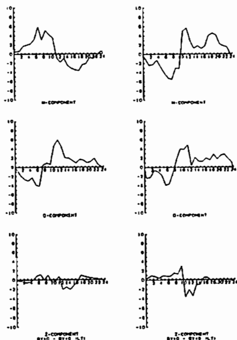
Fig. 1. Difference of the geomagnetic H (top), D (middle) and Z (bottom) components when IMF-By > 0 and < 0 at Boulder (geomagnetic lat. 49^{\circ} N, left) and Argentine Island ( 54^{\circ} S, right) in 1980.
