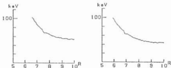
Fig.3 Profiles of Fig.2 for protons of 0.7keV/nT, 90^\circ and 60^\circ at 1800LT.
