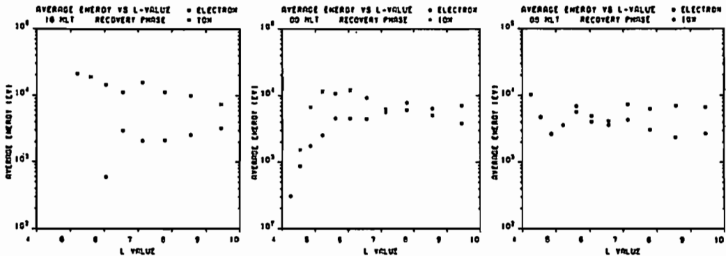
Fig. 1 Dependences of electron and ion average energy upon L-value in substorm recovery phase (~0.5-2 hour after substorm onset). The average energies are estimated from DMSP particle data and averaged within \pm 1 hour for each MLT. (See the simulation results of Fig.14 in Ejiri et al., 1980.)
