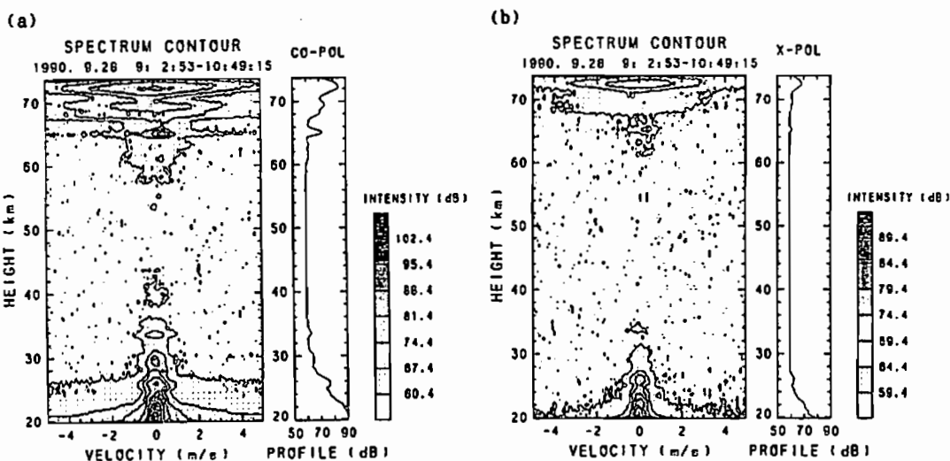
Fig.1 Spectrum contours of Doppler velocities received by (a) co-pol and (b) x-pol arrays.
