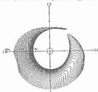
Fig.1 Proton trajectories mapped on the equatorial plane (0.7keV/nT, 60^\circ )
