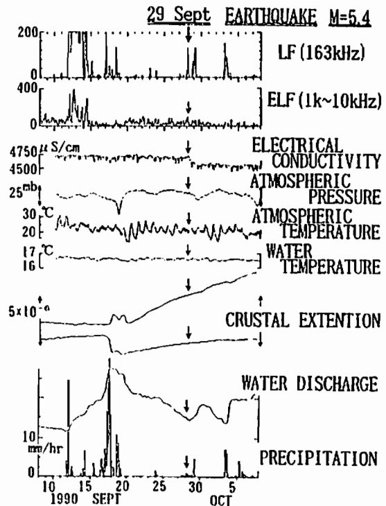
Fig. Hourly numbers of electromagnetic pulse type noises on LF and ELF ranges and the variations of the other geophysical phenomena accompanied with the Western Hyogo Prefecture Earthquake with magnitude 5.4, occurred on 29 Sept. 1990, near active Yamasaki Fault with focal depth of 12km, determined by J.M.A..
