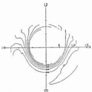
Fig.2 Kinetic energy contour of drifting protons of 0.7 keV/nT, 60^\circ .
