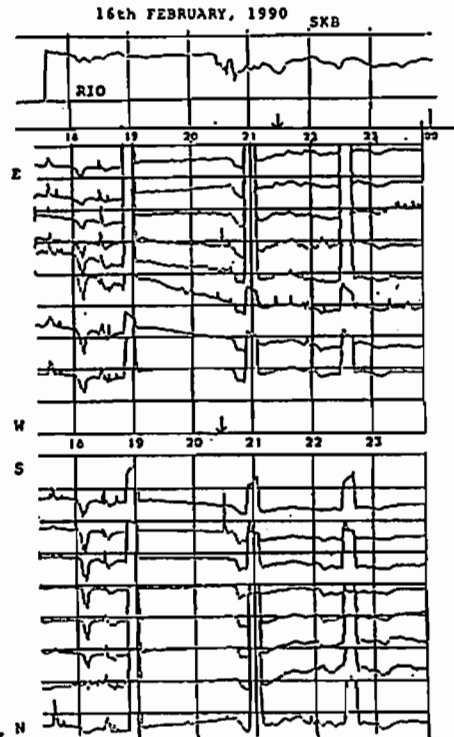
CNA events observed at Skibotn and Ny-Alesund.
