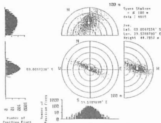
Fig.1 Scatter plots of fixed position from the mean position of the Earth Science Laboratory. The center was derived by averaging data except unusual cases. Data for r \leq 100 and GDOP \leq 5 are plotted and used for deriving the mean value (open circle).
