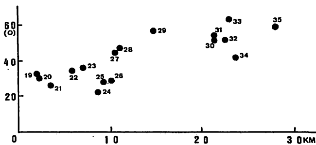
Fig. 2. Change in inclination of NRM of the dyke rocks with distance from the Median Tectonic Line.
