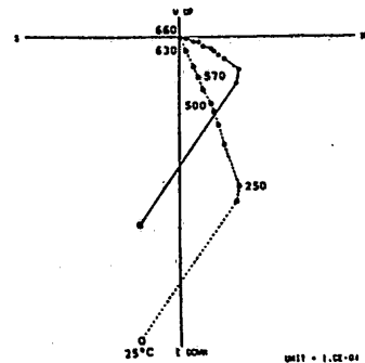
Runimidake rhyolitic tuff
