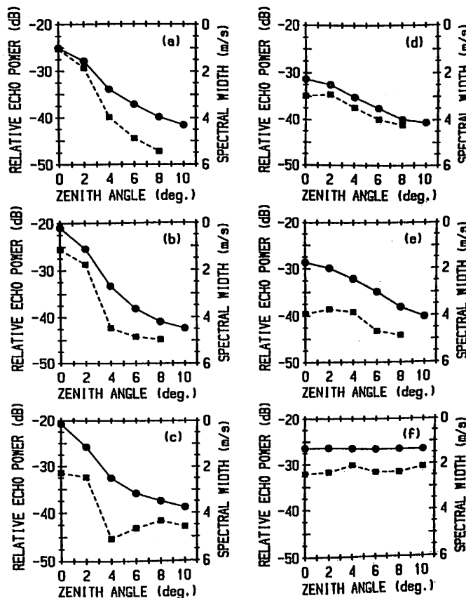
Fig. 1 Zenith angle dependence of P_1 (a circle) and 3 dB spectral width (a square) of the Doppler spectra averaged over 30 min., where \theta is the zenith angle in degree. Note that the vertical axis for the spectral width is plotted in the reverse direction. (a)-(e) correspond to stratospheric echoes, and (f) to a tropospheric echo.
